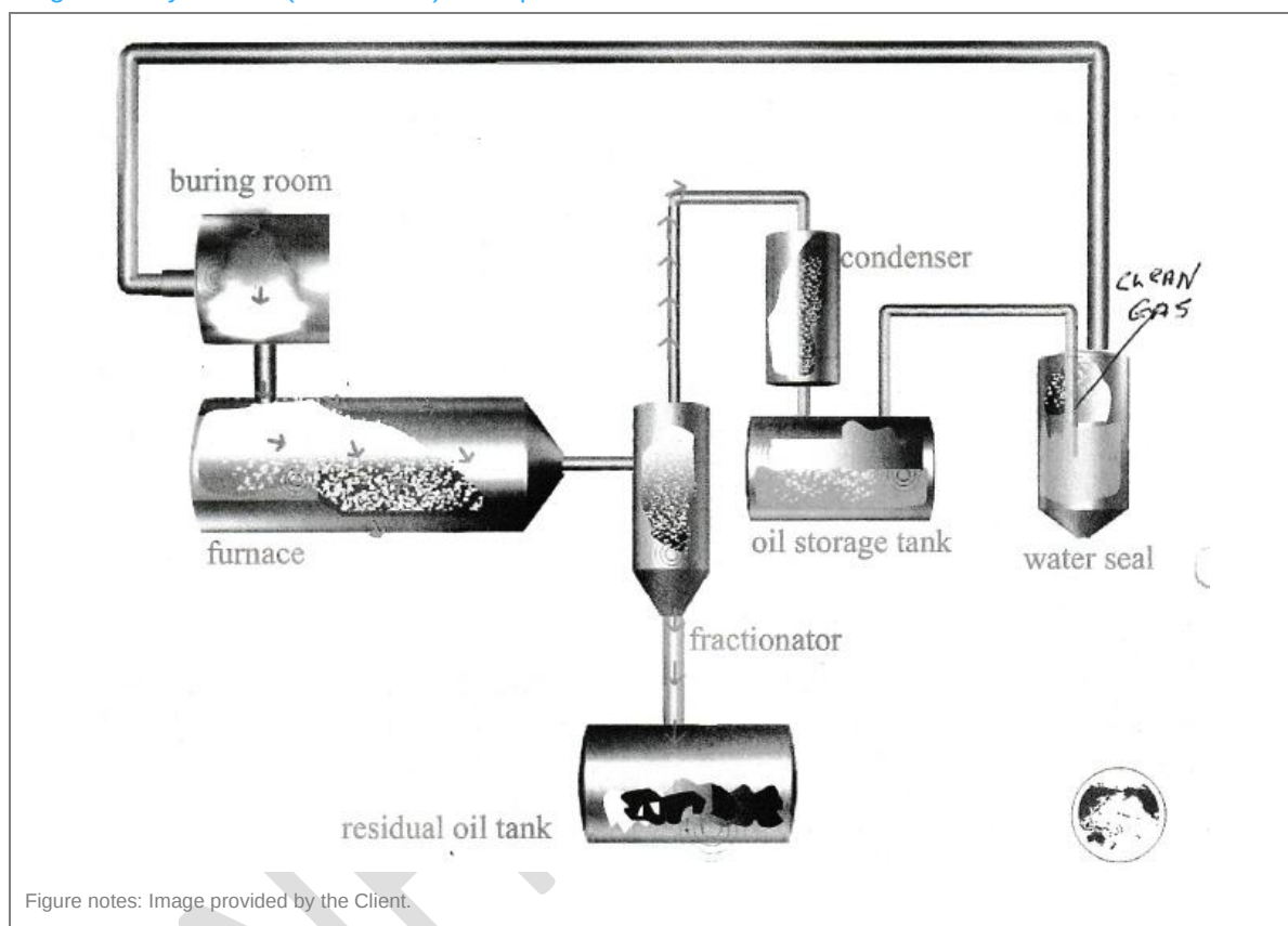
Figure 3: Hydroseal (Water seal) desulphurisation
