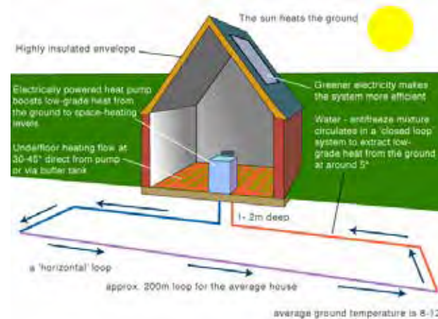
Above: Diagram of ground source heat loop system
