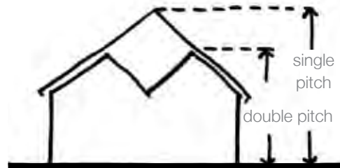
Above: illustration showing that using a double pitch reduces the overall building height
